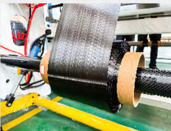
Unwinder
