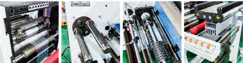
Magnetic Die Cutting Cylinder Rewinding Station Slitting Knives Web Guide System
