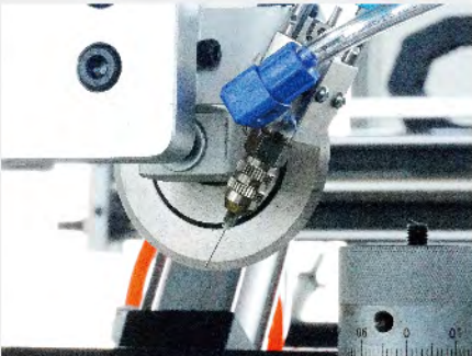
Cutter and Gluer
