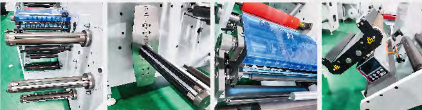
Rewinder 2pcs of 3"(76mm) Air Expanding Shafts Unwinder 3"(76mm) Air Expanding Shafts Slitting Knife with Safety Cover Web Guide
